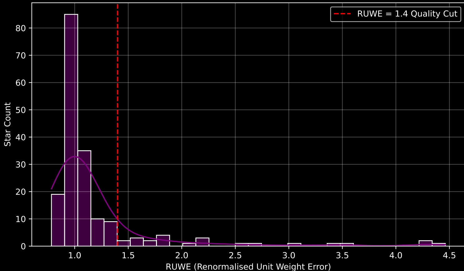
GAPOGEE DR17 Field [198+33_MGA] RUWE Distribution (n= 181)
