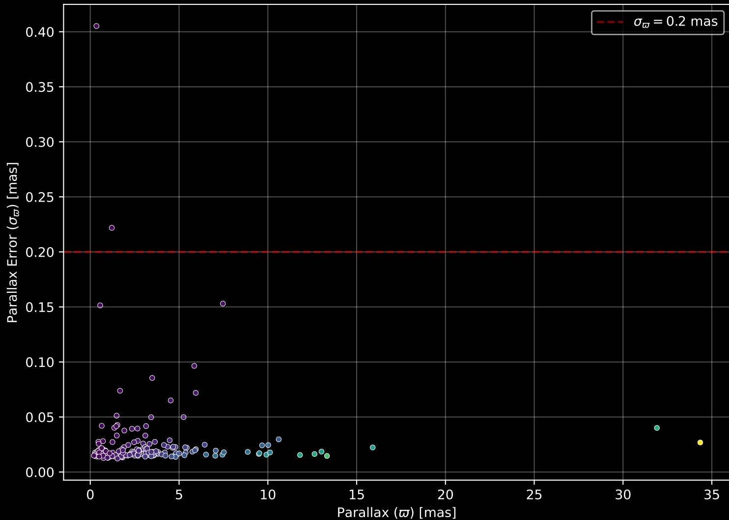
APOGEE DR17 Field: [198+33_MGA] Parallax Quality (n= 186)
