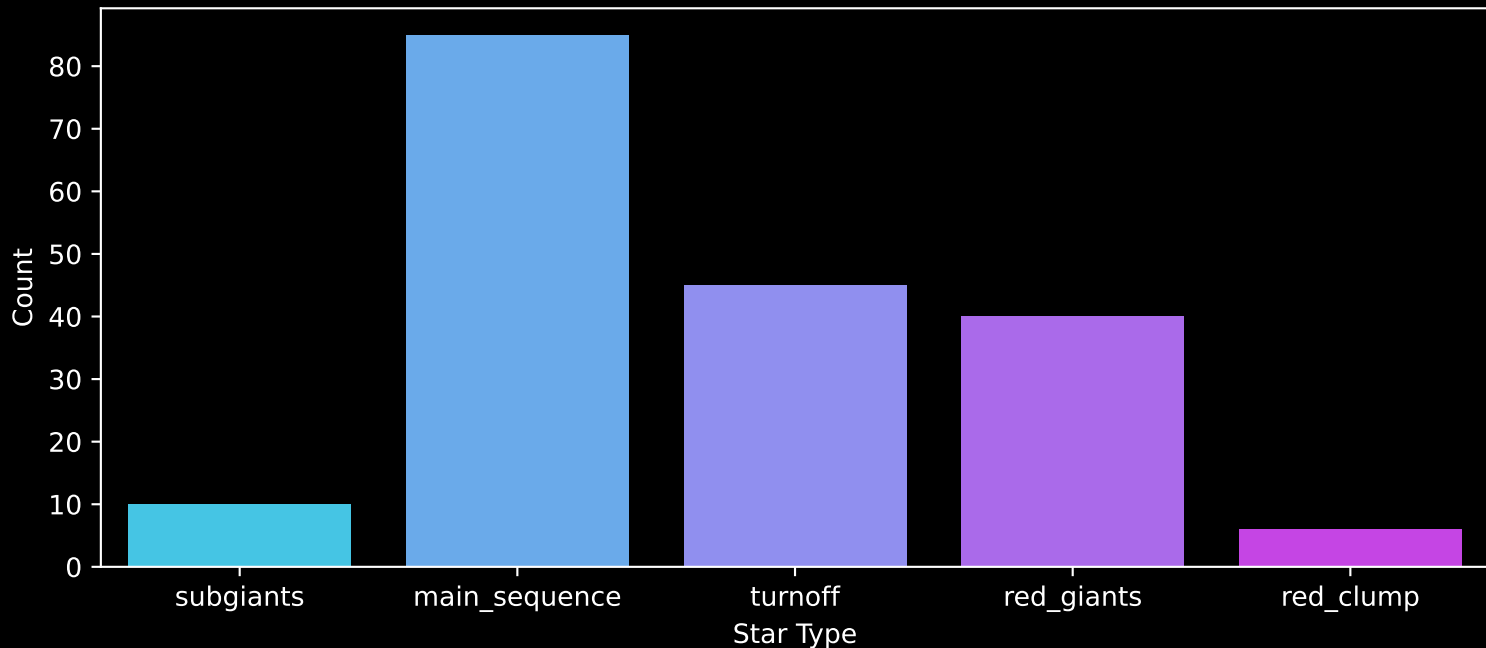
APOGEE DR17 Field: [198+33_MGA] Count plot of Star Type
