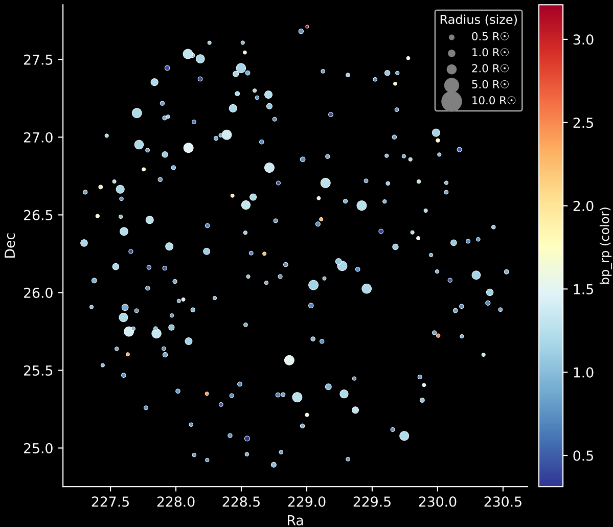
APOGEE DR17 Field: [198+33_MGA] Stars: 186
