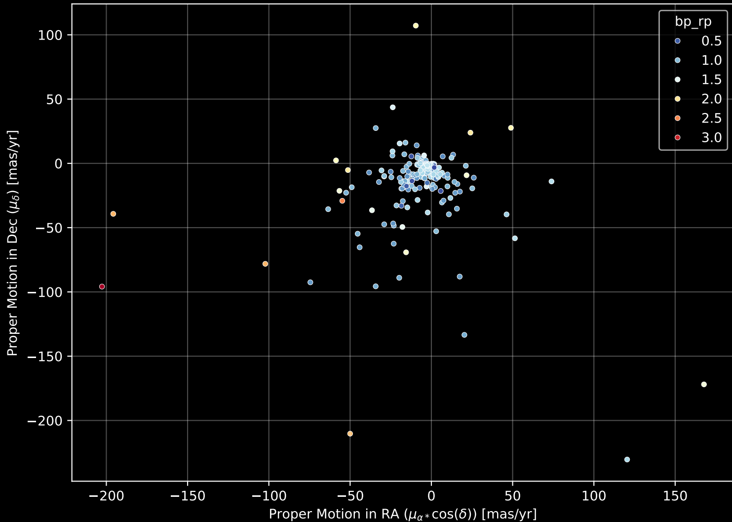
APOGEE DR17 Field: [198+33_MGA] Proper Motion Diagram (n= 186)
