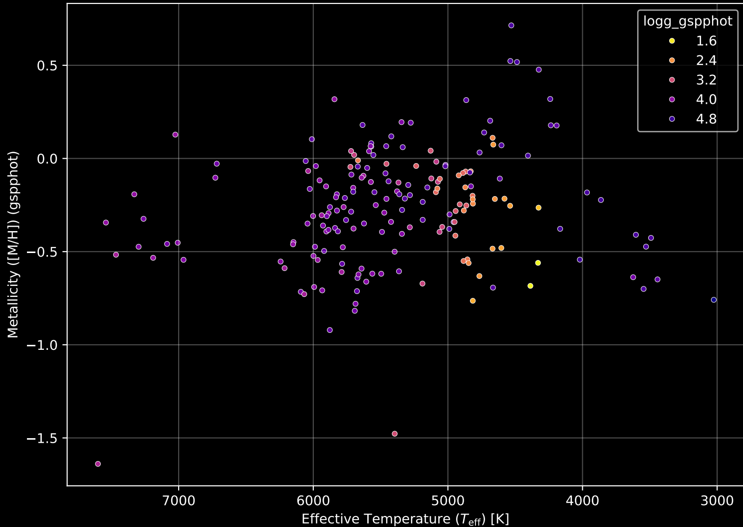
APOGEE DR17 Field: [198+33_MGA] Stellar Population Parameters (n= 186)
