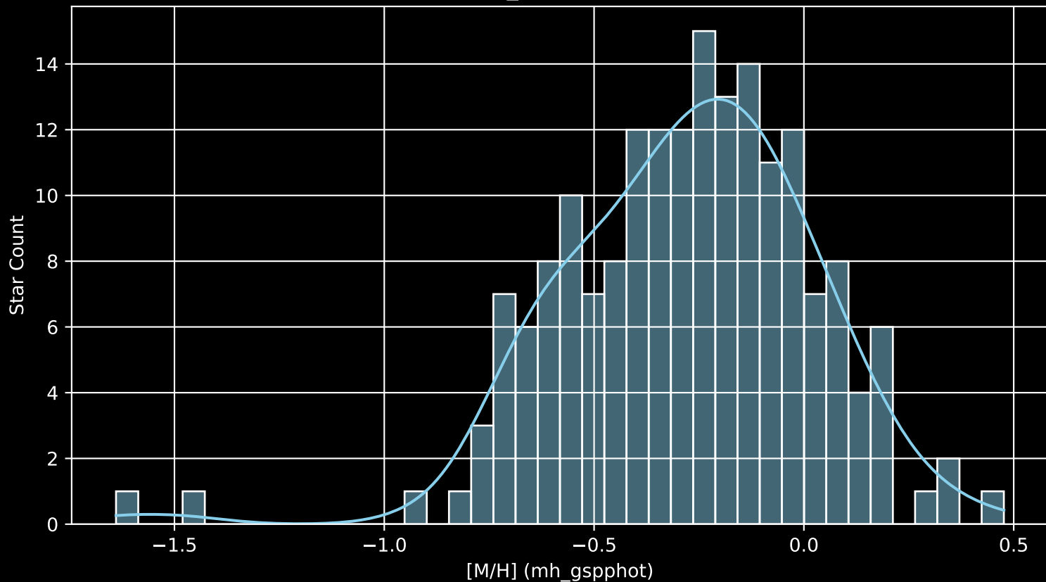
APOGEE DR17 Field: [198+33_MGA [M/H] (mh_gspphot) (n= 183)
